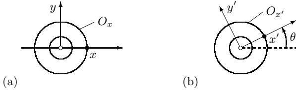
Fig. 16.1. Symmetry and orbits
