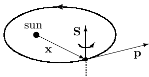
Fig. 2.16. Spin of a planet
