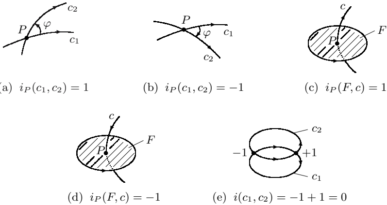
Fig. 5.4. Intersection number
