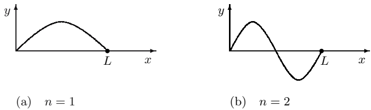
Fig. 2.3. Standing waves
