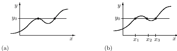
Fig. 5.9. Sard's theorem
